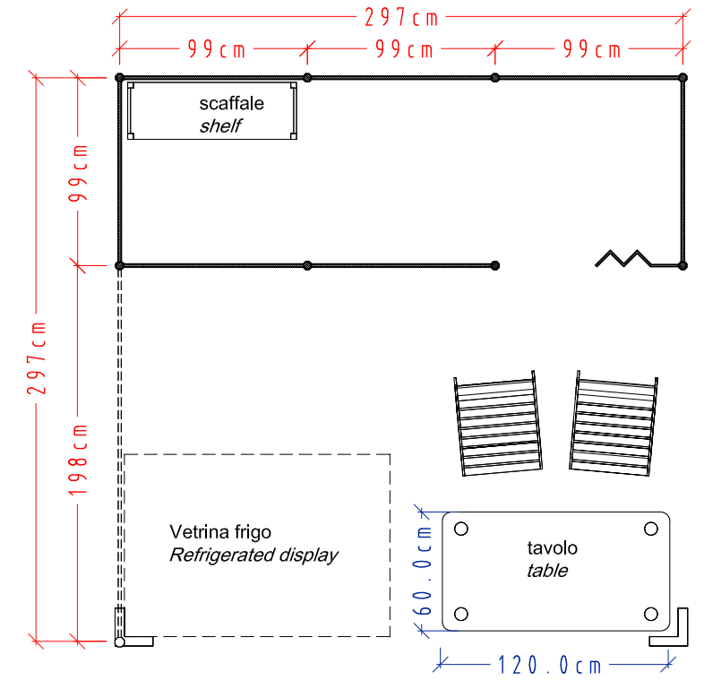
PLANIMETRIA/PLAN
